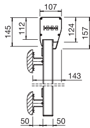
Wall fixing with square box Montaje a pared con cofre angular
