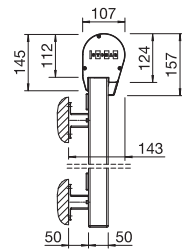
Wall fixing with round box Montaje a pared con cofre redonda
